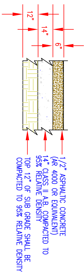
TYPICAL CROSS SECTION FOR ARTERIAL STREET DETAIL "A"
