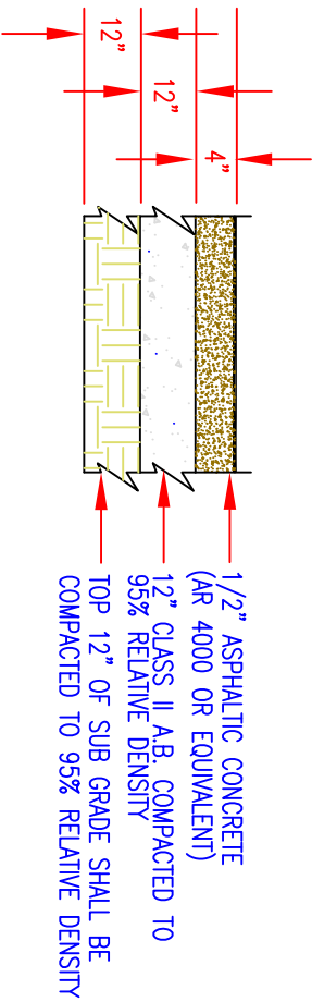
TYPICAL CROSS SECTION FOR A COLLECTOR STREET DETAIL "B"
